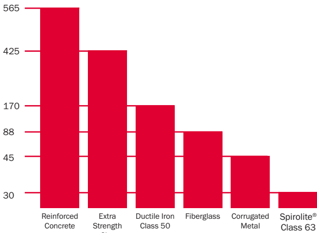
FIGURE 2: TYPICAL WEIGHT OF 36" SEWER PIPE
